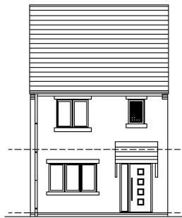
PROPOSED FRONT ELEVATIONS
