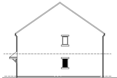
PROPOSED SIDE ELEVATIONS
