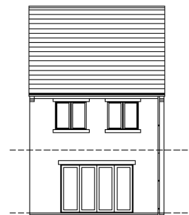
PROPOSED REAR ELEVATIONS
